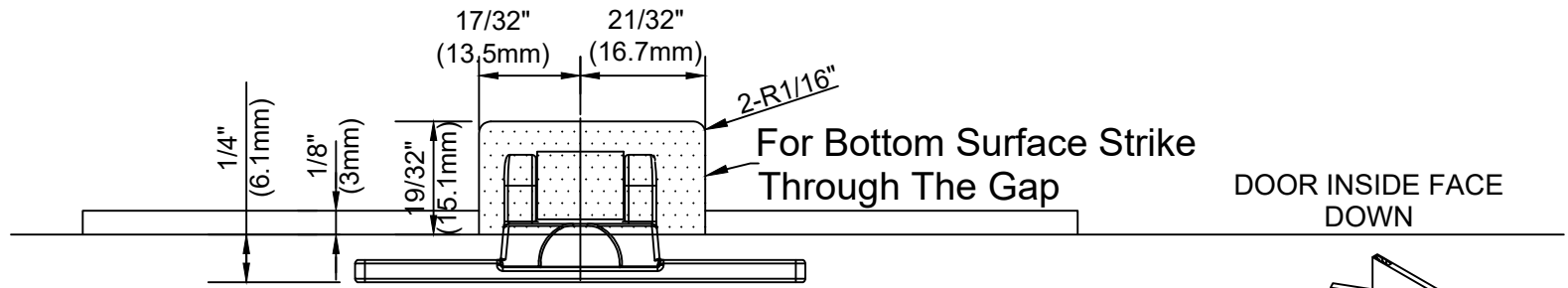
TEMPLATE of Bottom Latch Housing Ass'y [ Bottom Mounting Plate (regular use)]
